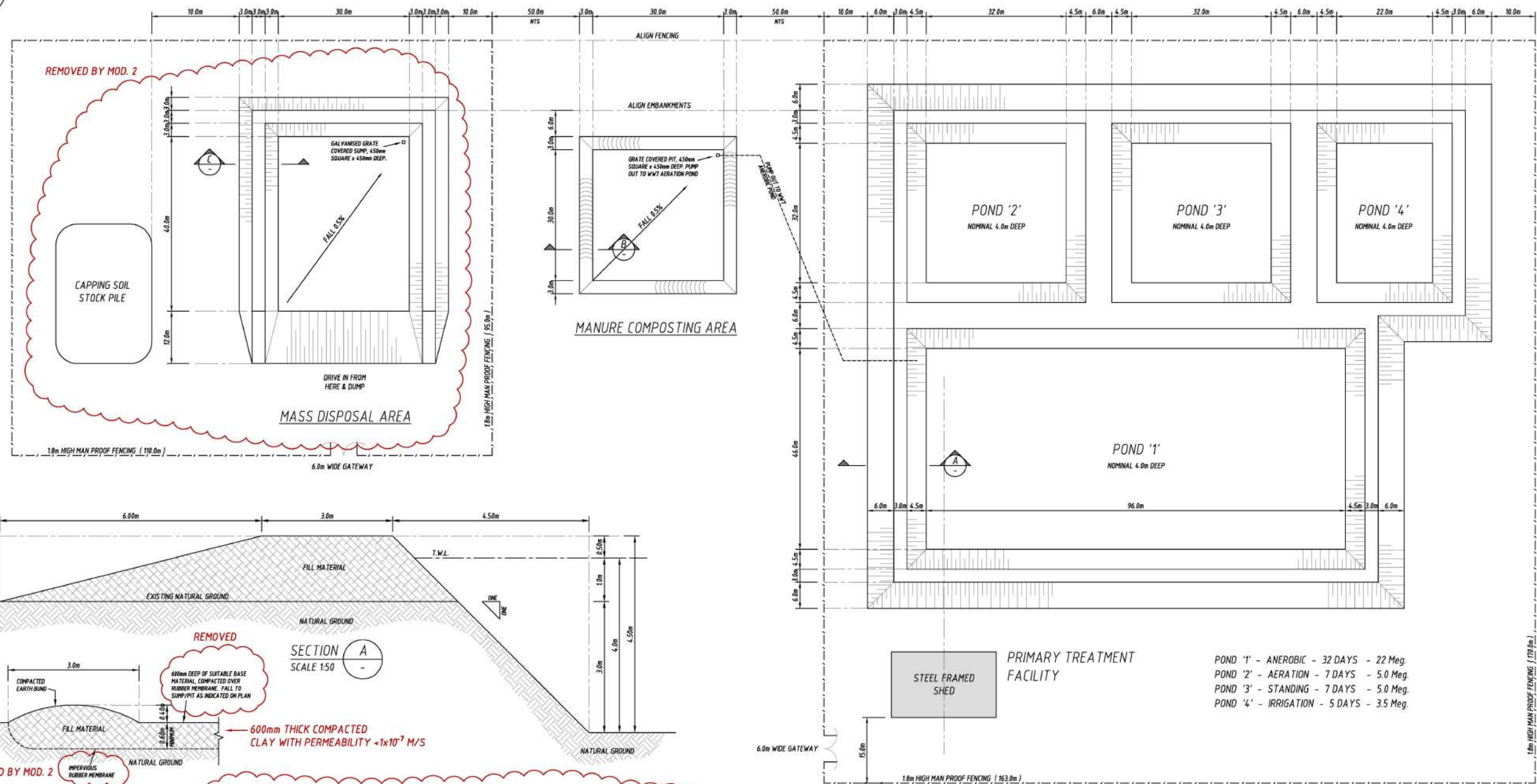
EVAPORATION PONDS PLANS OF EVAPORATION PONDS, MANURE COMPOSTING & TIP AREAS SCALE 1:500
