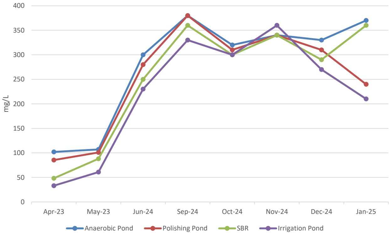
Nitrogen Total
