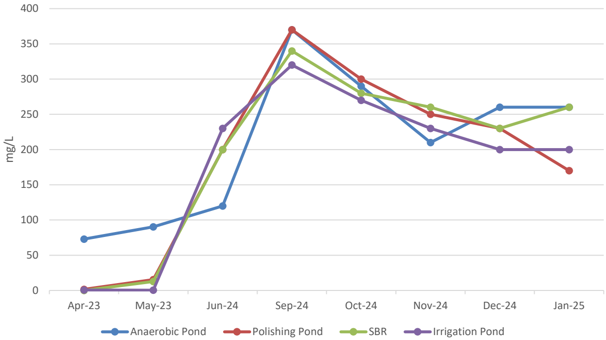
Nitrogen Ammonia
