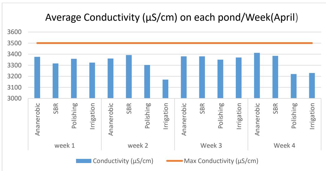
Figure 6: TFI Bourke abattoir average conductivity of effluent weekly testing.
