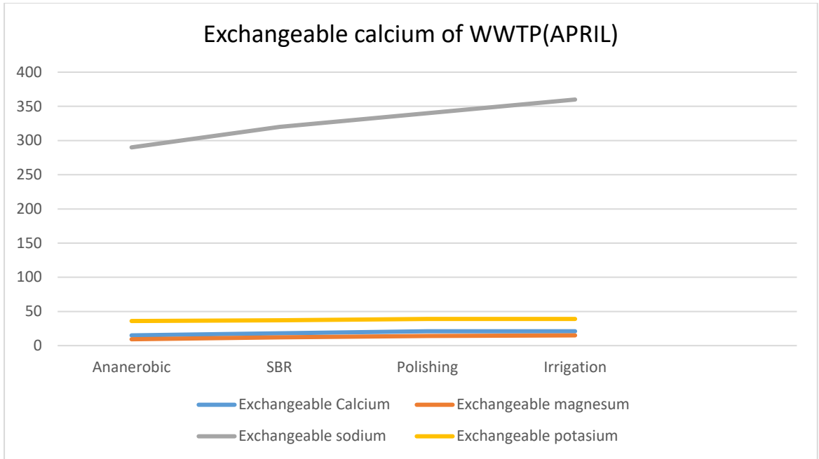
Figure 15: TFI Bourke abattoir exchangeable calcium of effluent monthly testing.
