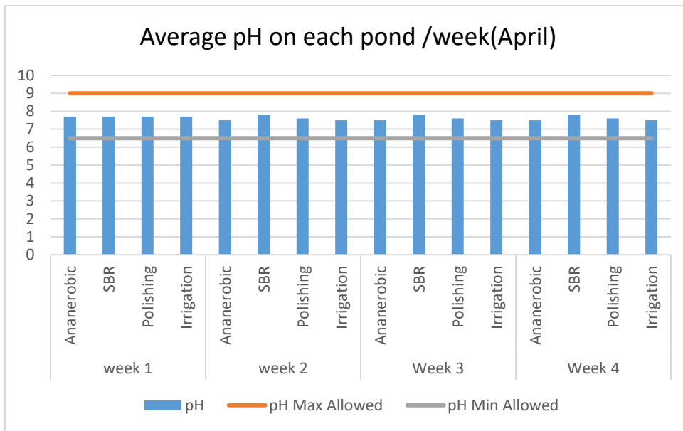
Figure 5: TFI Bourke abattoirs pH weekly testing results of effluent
