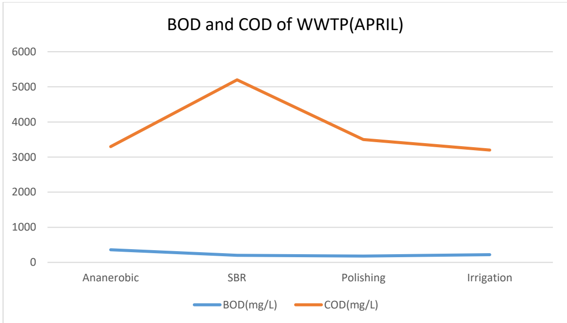
Figure 11: TFI Bourke abattoir BOD and COD of effluent monthly testing.
