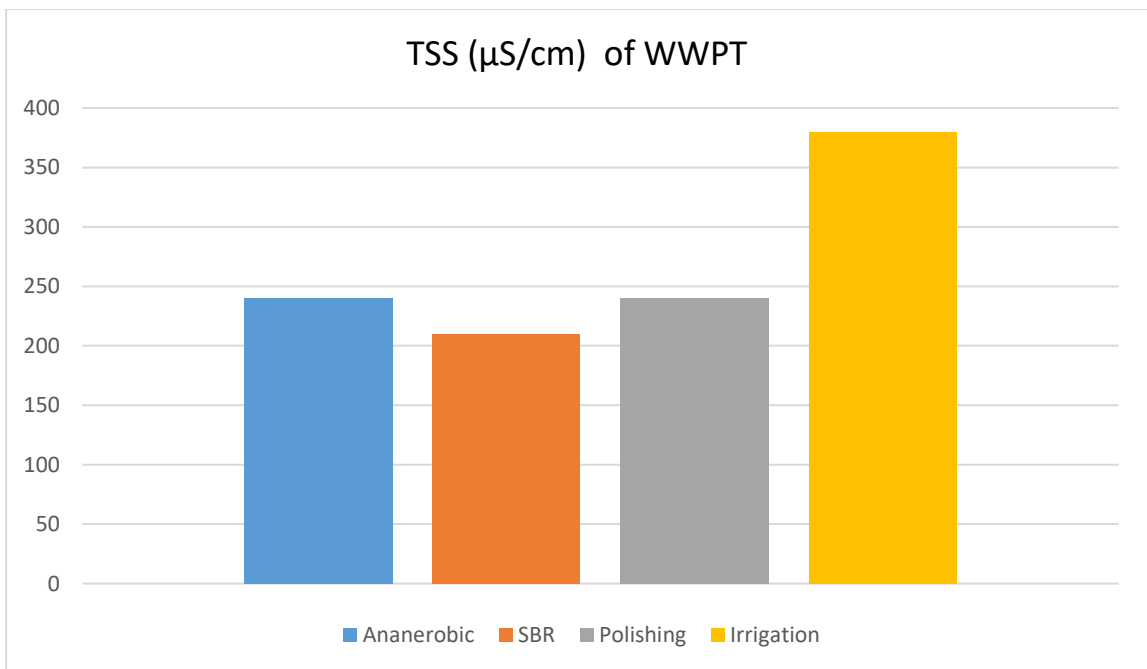
Figure 10: TFI Bourke abattoir average TSS of effluent monthly testing.
