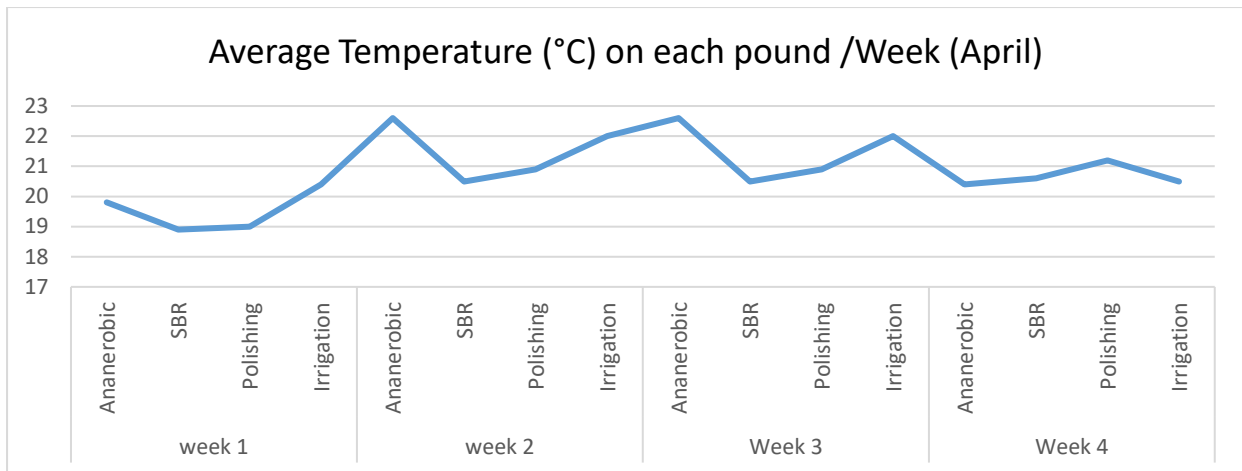
Figure 7: TFI Bourke abattoir average temperature of effluent weekly testing.
